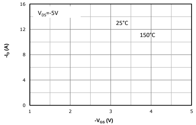
Fig 2: Transfer Characteristics
